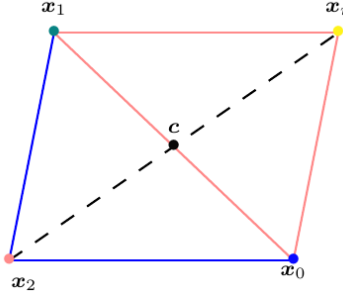
Figure 11.6: x_2 is mirrored in c and creates a reflected point x_r .
