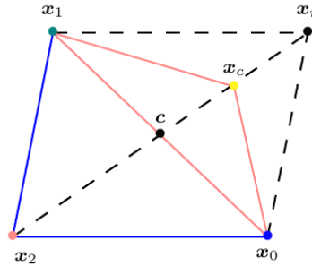
Figure 11.8: The contraction point x_c^{out} is computed outside the old simplex.
