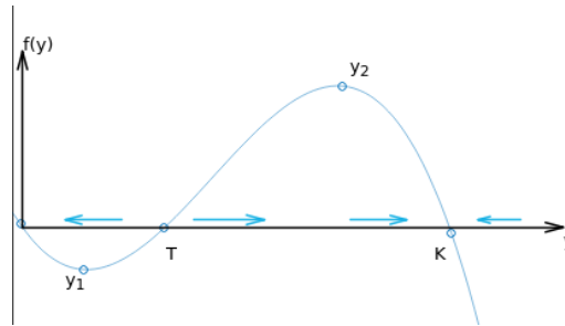
Figure 5.28: The graph of f(y) versus y for logistic growth with a threshold for \frac{dy}{dt} = -r \left(1 - \frac{y}{T}\right) \left(1 - \frac{y}{K}\right) y (Hamzstplot/Examples with Makefile/Plot 2D Equilibrium Solution for Logistic Growth with a Threshold/main.cpp).
