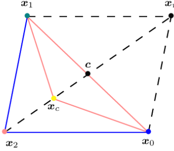
Figure 11.9: The contraction point x_c^{in} is computed inside the old simplex.
