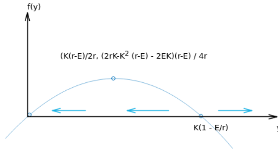
Figure 5.30: The equilibrium points and the stability analysis for \frac{dy}{dt} = f(y) = \left(y - K\left(1 - \frac{E}{r}\right)\right)y (Hamzstplot/Examples with Makefile/Plot 2D Equilibrium Solution for Schaefer Model/main.cpp).
