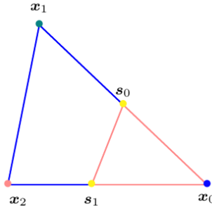
Figure 11.10: Shrink the simplex by moving every point closer to the current best.
