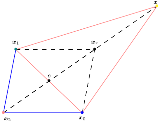
Figure 11.7: The expansion point x_e is computed by moving further away from c .
